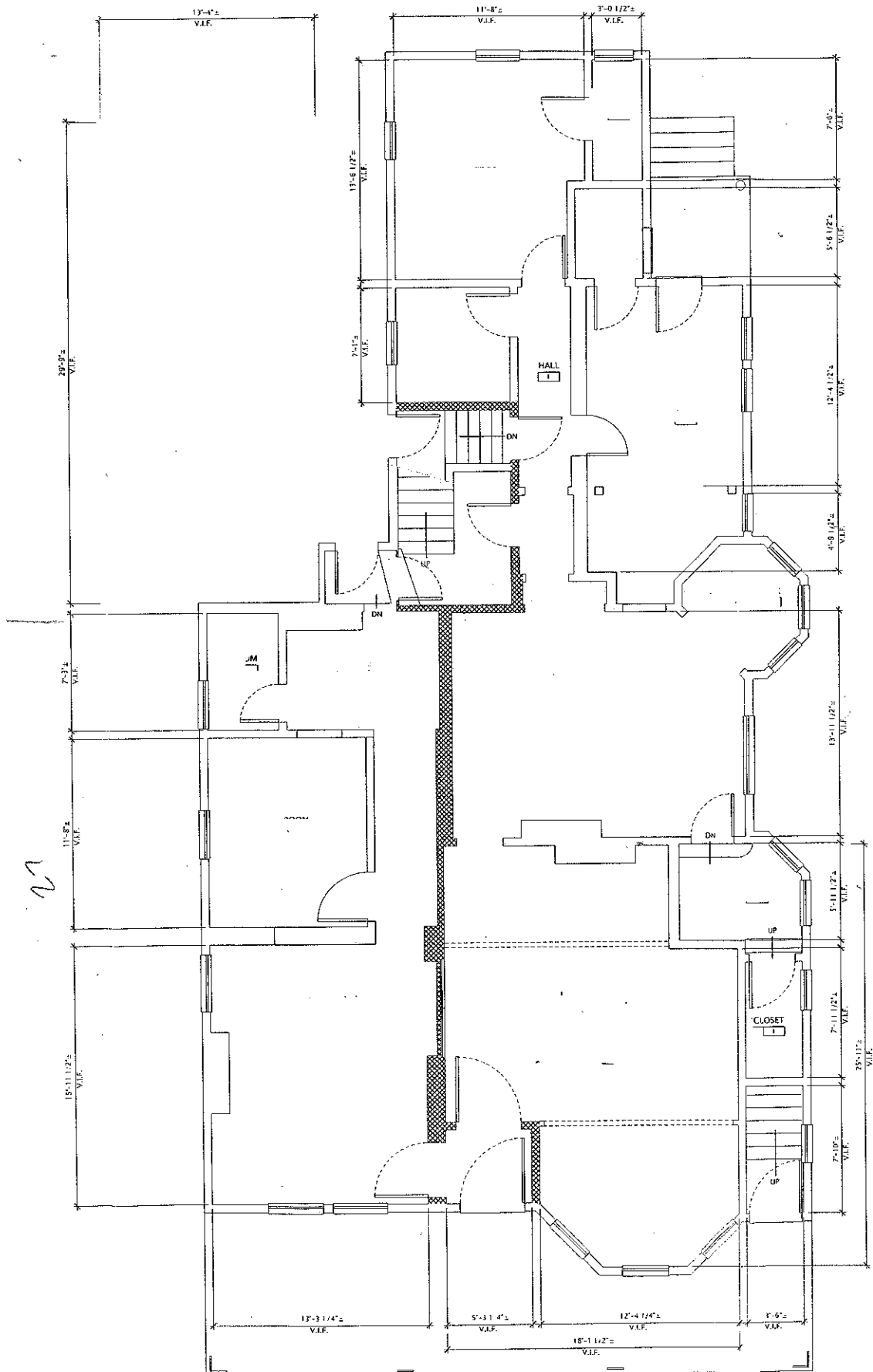
1 FIRST FLOOR PLAN 1/4" = 1'-0"
