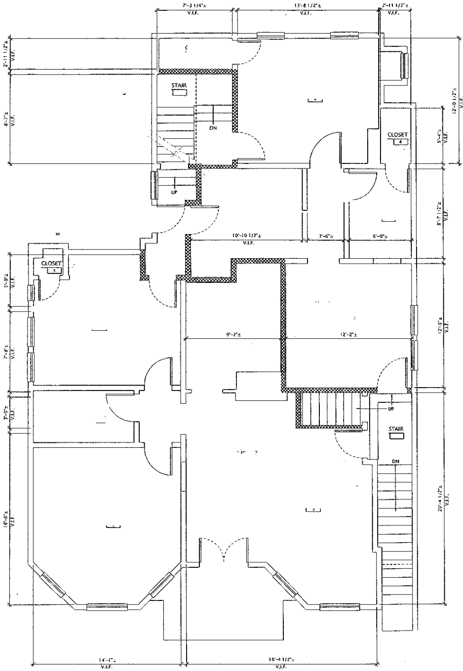
2 SECOND FLOOR PLAN A1.1 1/4" = 1'-0"
